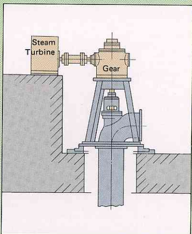
Steam turbine drive
