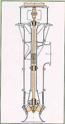
Pull-out type (Low head) Model "VZN"
