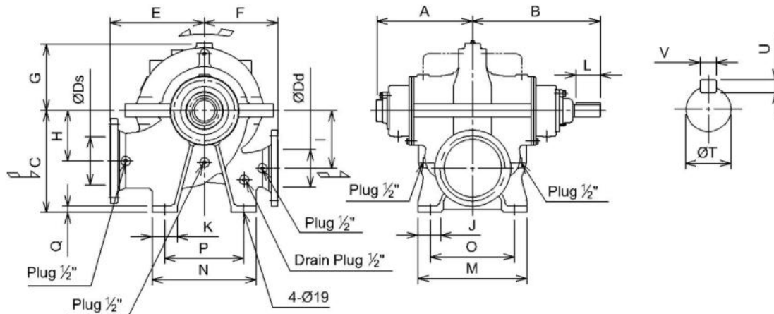
Horizontal Split Case Pump
