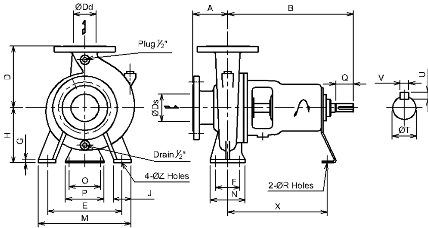
End Suction Pump
