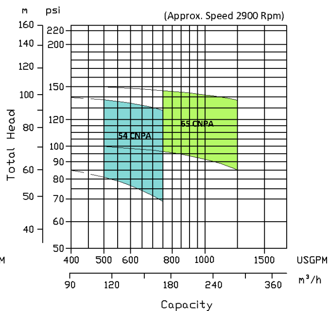
Split Case Pump
