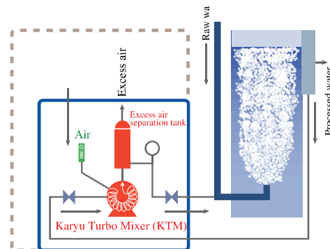
Karyu Turbo Mixer/KTM (with automatic air suction mechanism)
